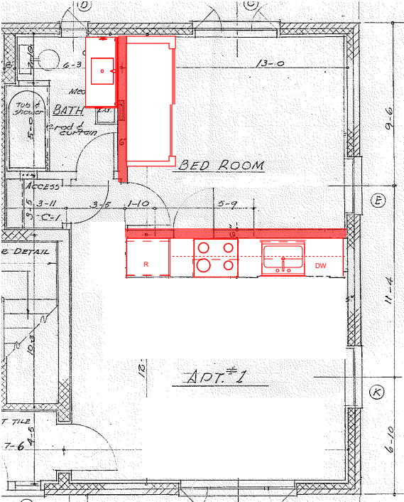
Typical One Bed Unit Renovation 468 SF
