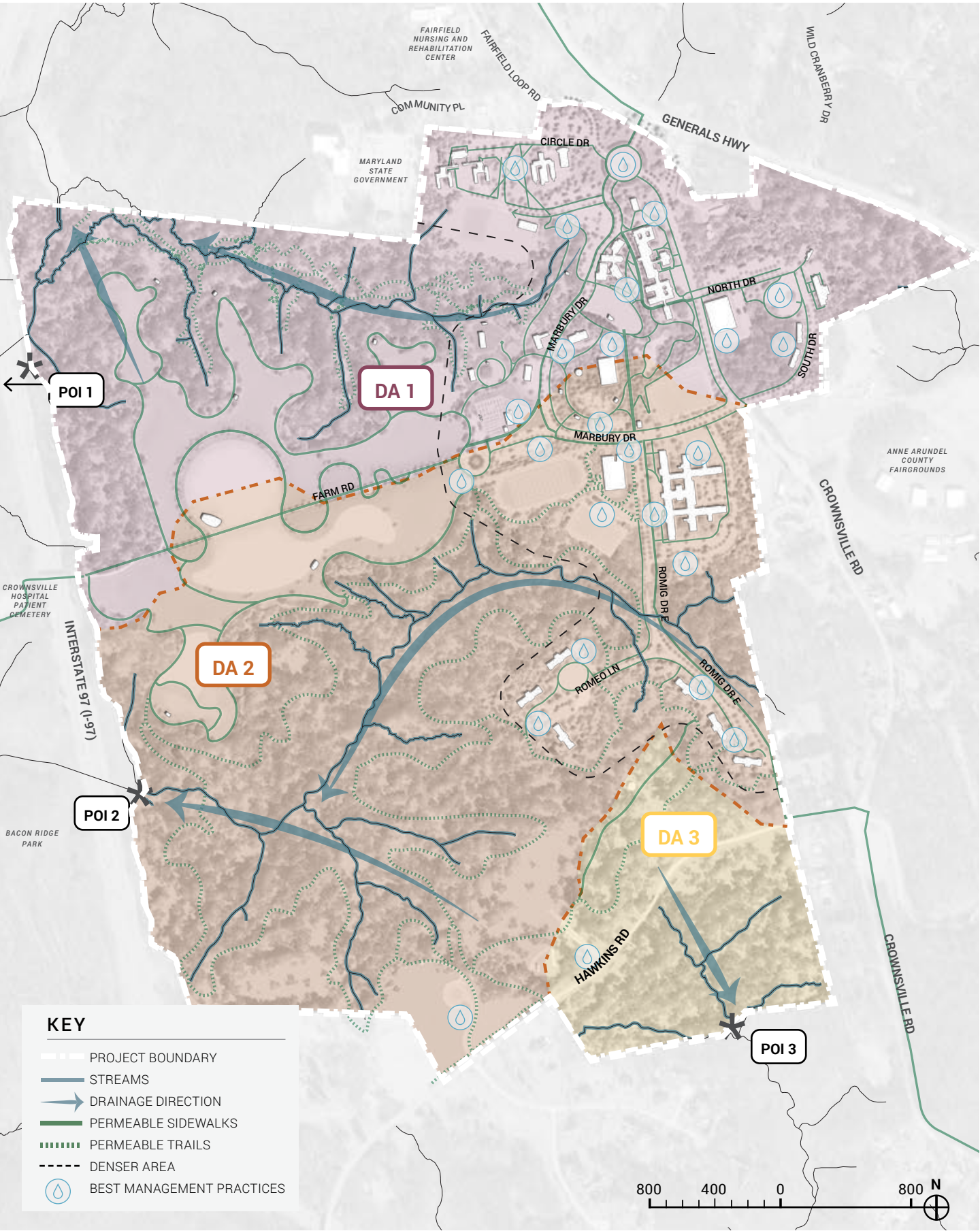
Hydrology Plan | Source: RK&K/Design Collective All images and plans are for illustrative purposes and subject to change.
