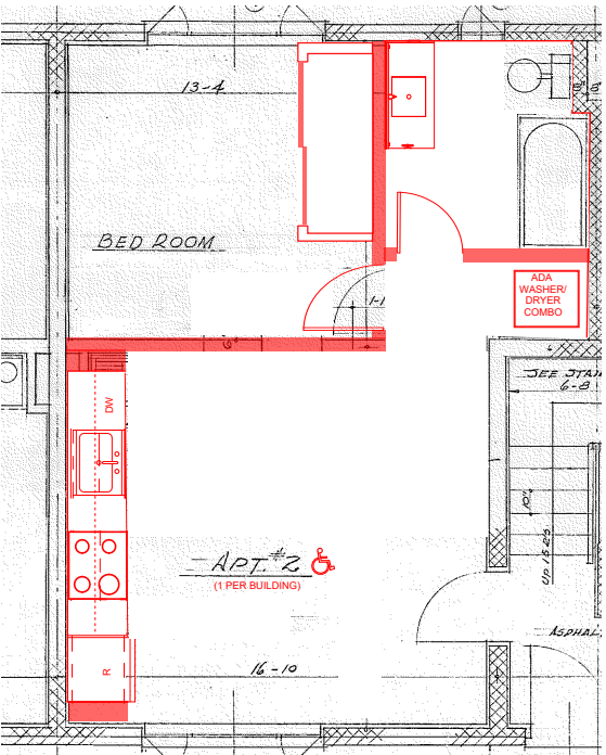
Typical ADA One Bed Unit Renovation 468 SF
